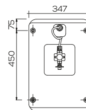
V. TRASERA
