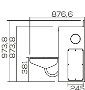
V. LATERAL
