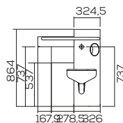
V. FRONTAL
