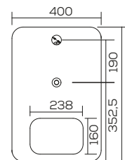
V. FRONTAL
