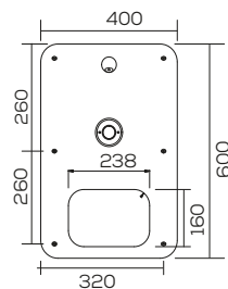
V. FRONTAL
