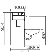
V. LATERAL
