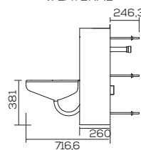
V. LATERAL
