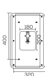
V. TRASERA
